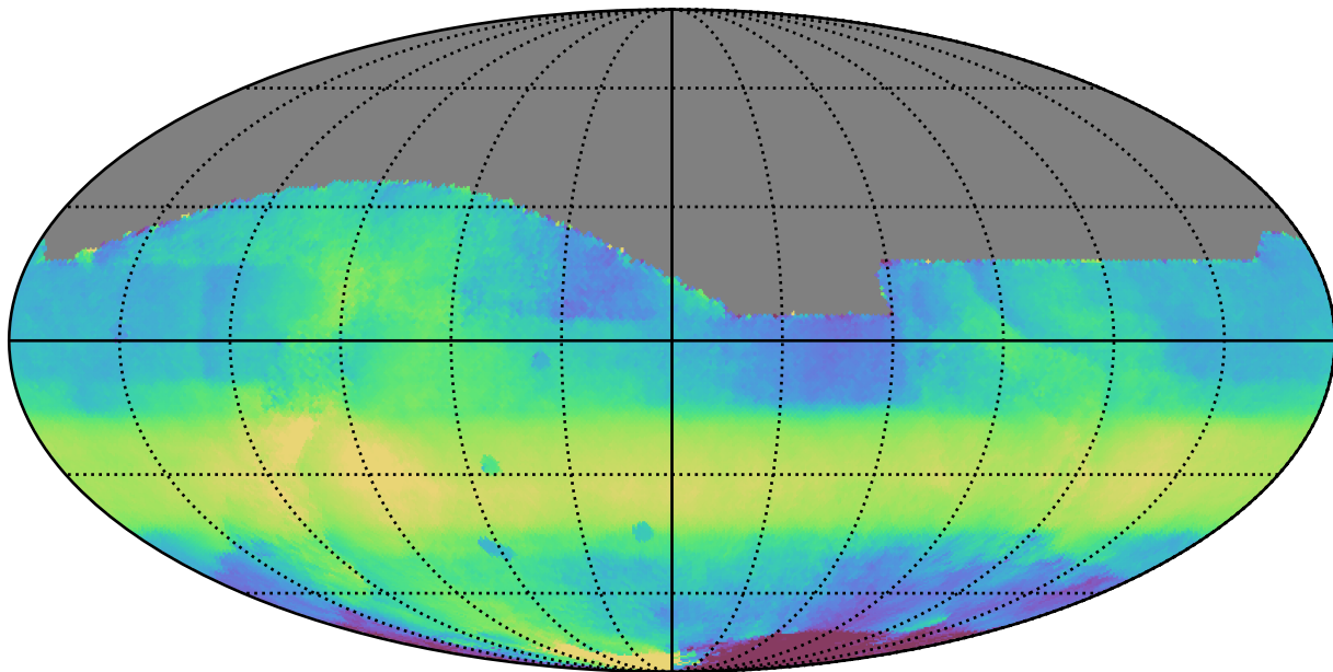
ddf_acor_sf15_lsf30_lsr50_v3.4_10yrs All sky all bands: Median HA
