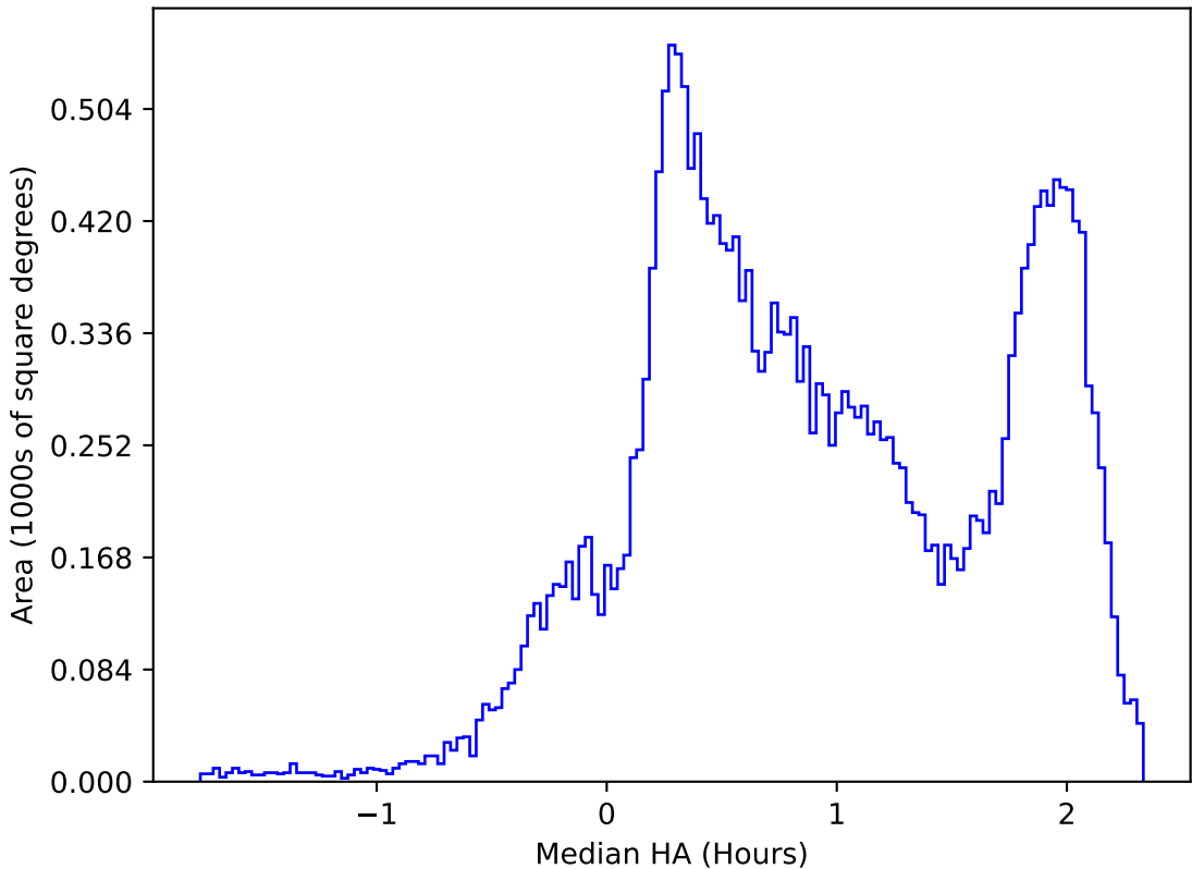
ddf_acor_sf15_lsf30_lsr50_v3.4_10yrs All sky all bands: Median HA
