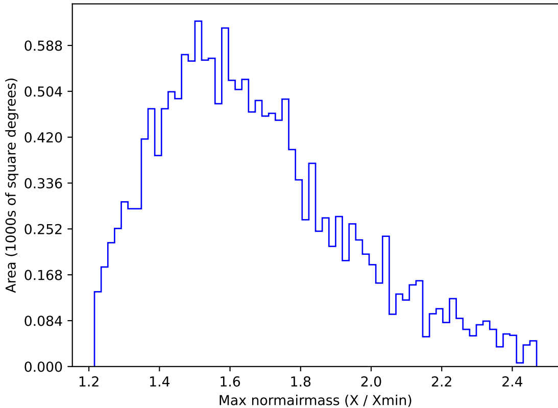
ddf_acor_sf15_lsf30_lsr50_v3.4_10yrs WFD u band: Max normairmass
