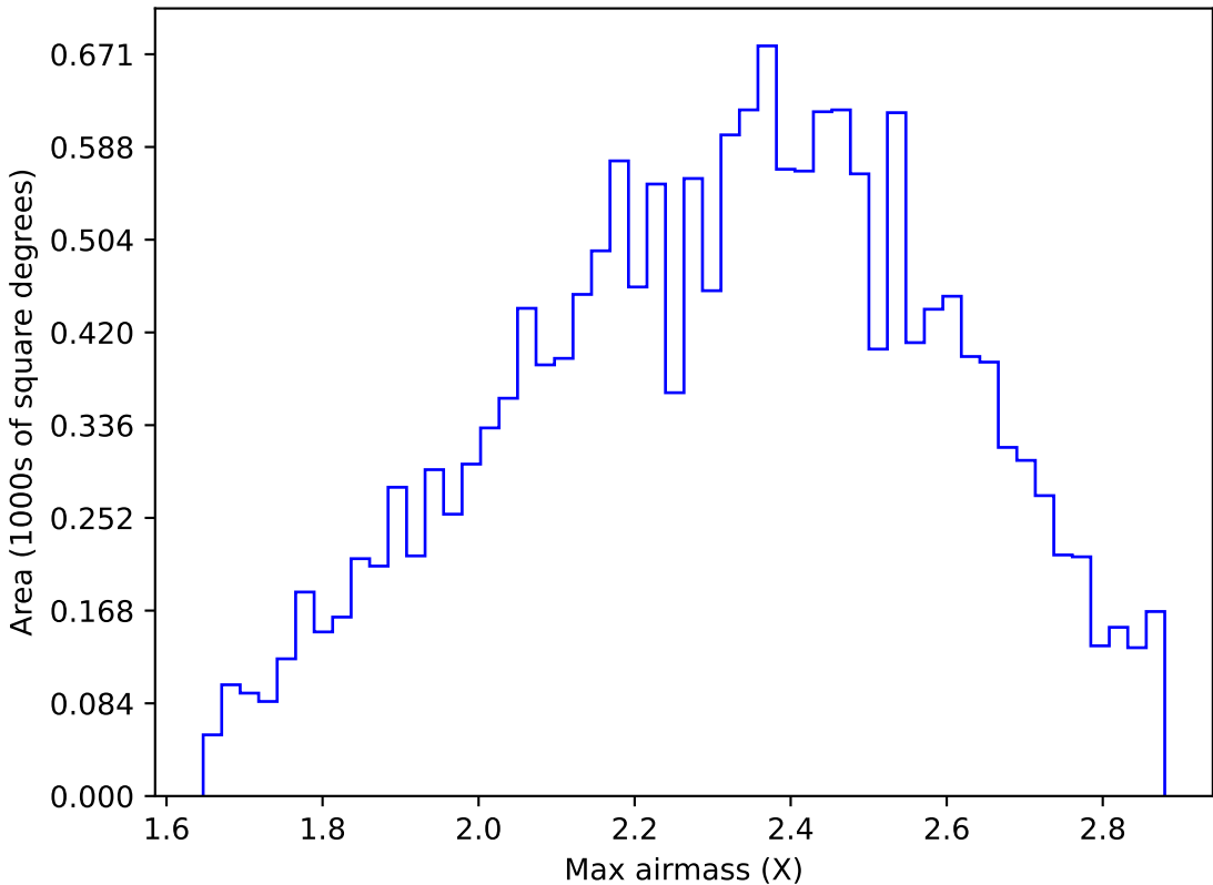
ddf_acor_sf15_lsf30_lsr50_v3.4_10yrs WFD y band: Max airmass
