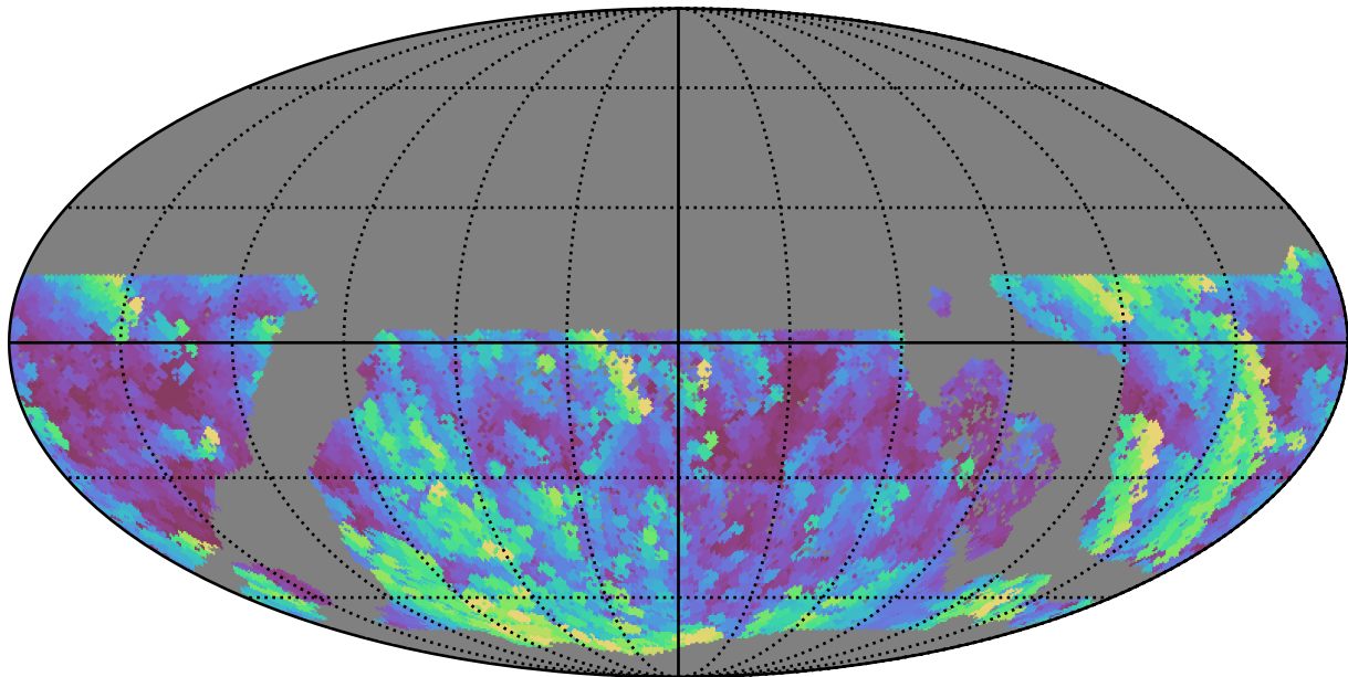
ddf_acor_sf15_lsf30_lsr50_v3.4_10yrs WFD u band: Max airmass
