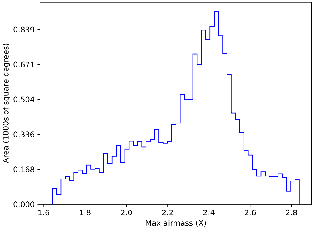
ddf_acor_sf15_lsf30_lsr50_v3.4_10yrs WFD r band: Max airmass
