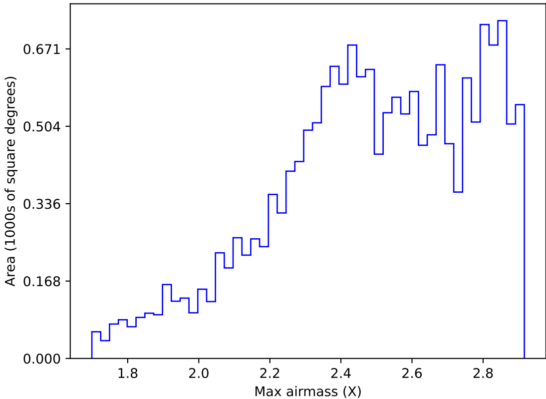
ddf_acor_sf15_lsf30_lsr50_v3.4_10yrs WFD i band: Max airmass
