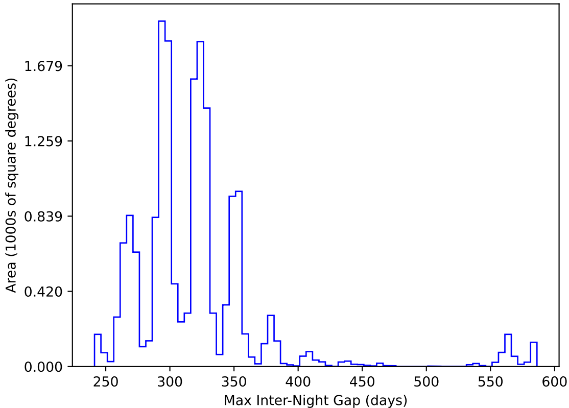
ddf_acor_sf15_lsf30_lsr50_v3.4_10yrs WFD y band: Max Inter-Night Gap
