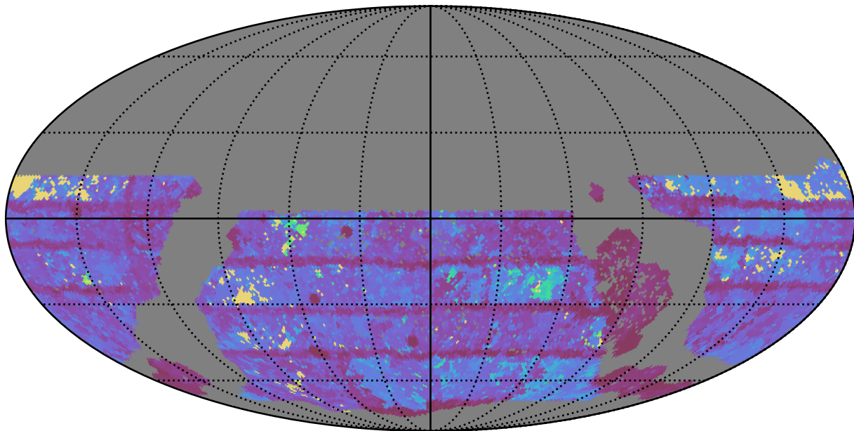
ddf_acor_sf15_lsf30_lsr50_v3.4_10yrs WFD r band: Max Inter-Night Gap
