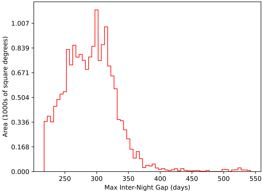
ddf_acor_sf15_lsf30_lsr50_v3.4_10yrs WFD i band: Max Inter-Night Gap
