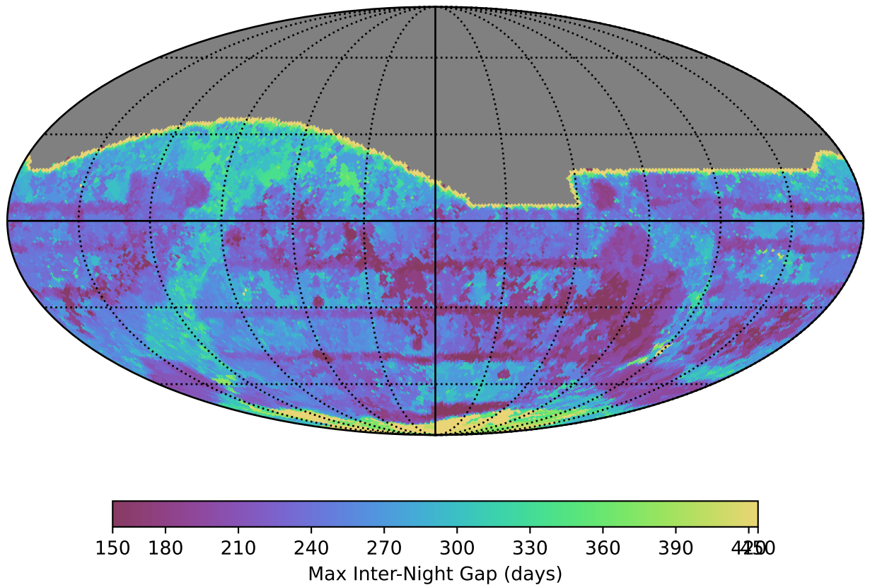
ddf_acor_sf15_lsf30_lsr50_v3.4_10yrs All sky all bands: Max Inter-Night Gap
