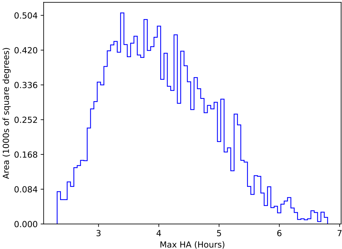
ddf_acor_sf15_lsf30_lsr50_v3.4_10yrs WFD g band: Max HA
