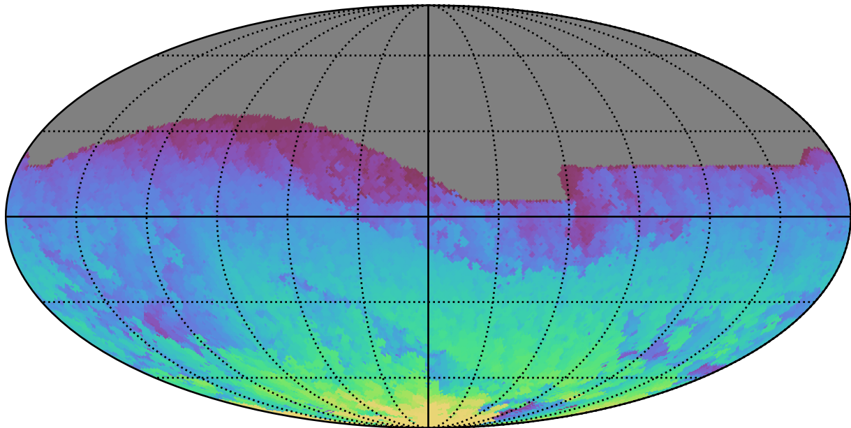
ddf_acor_sf15_lsf30_lsr50_v3.4_10yrs All sky z band: Max HA
