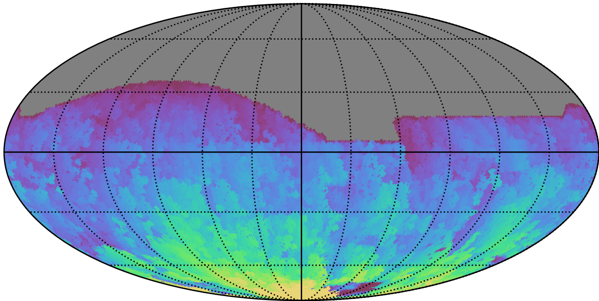
ddf_acor_sf15_lsf30_lsr50_v3.4_10yrs All sky r band: Max HA
