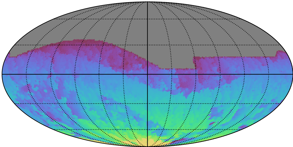
ddf_acor_sf15_lsf30_lsr50_v3.4_10yrs All sky i band: Max HA
