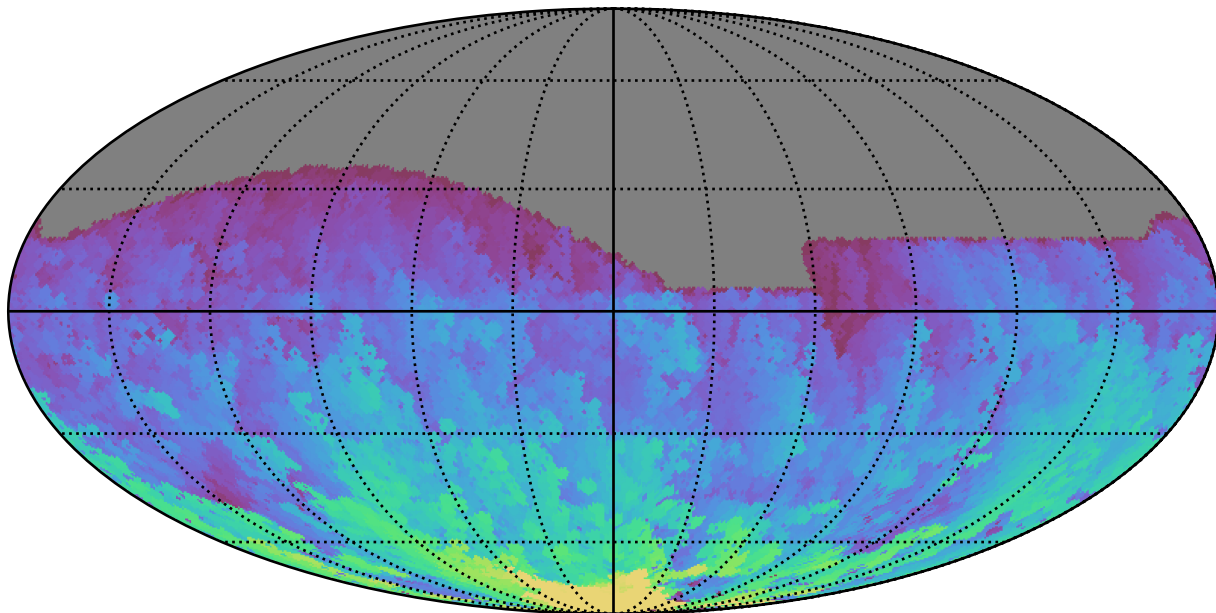
ddf_acor_sf15_lsf30_lsr50_v3.4_10yrs All sky g band: Max HA
