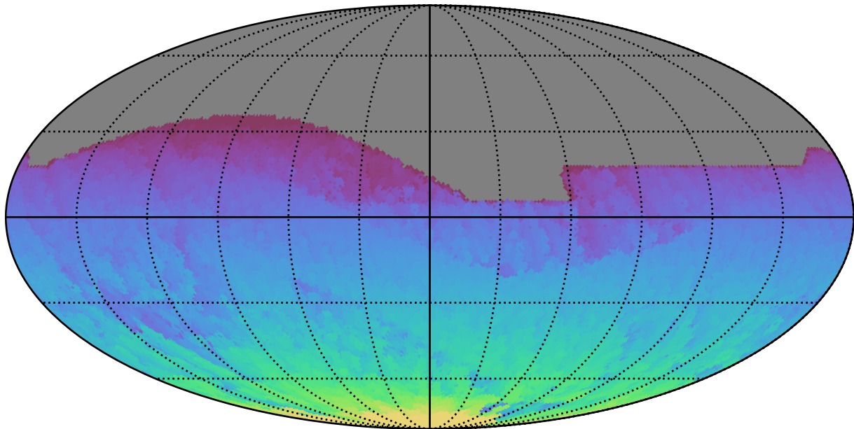
ddf_acor_sf15_lsf30_lsr50_v3.4_10yrs All sky all bands: Max HA
