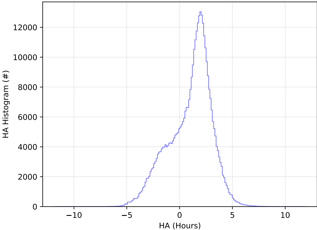
ddf_acor_sf15_lsf30_lsr50_v3.4_10yrs WFD y band: HA Histogram
