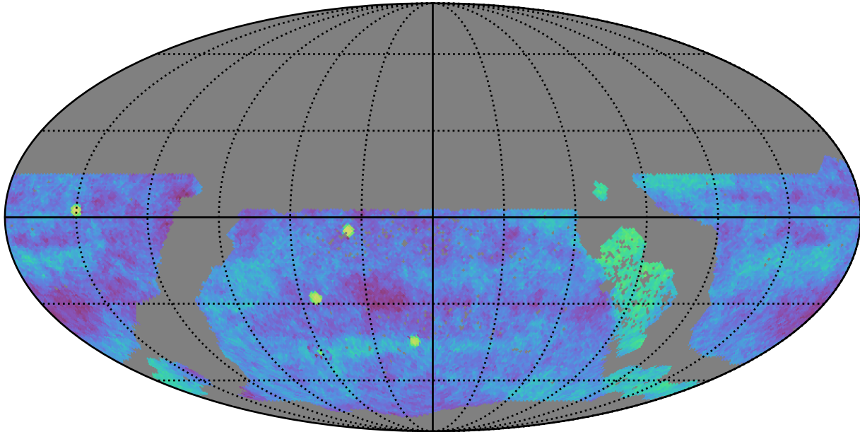
ddf_acor_sf15_lsf30_lsr50_v3.4_10yrs gri WFD: Fraction of visits in pairs (20-90 min)
