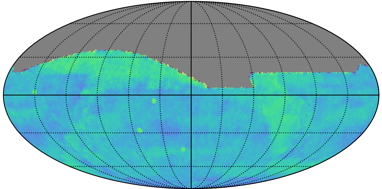
ddf_acor_sf15_lsf30_lsr50_v3.4_10yrs gri All sky: Fraction of visits in pairs (20-90 min)
