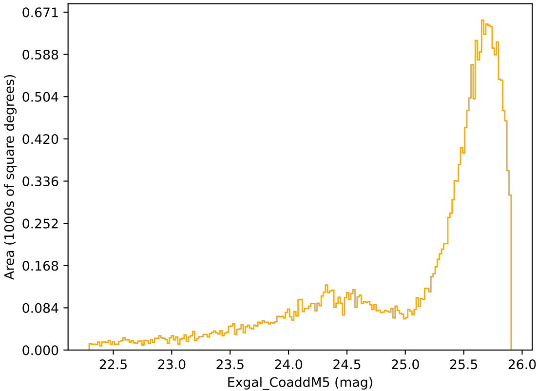
ddf_acor_sf15_lsf30_lsr50_v3.4_10yrs Yr 1 r band: Exgal_CoaddM5
