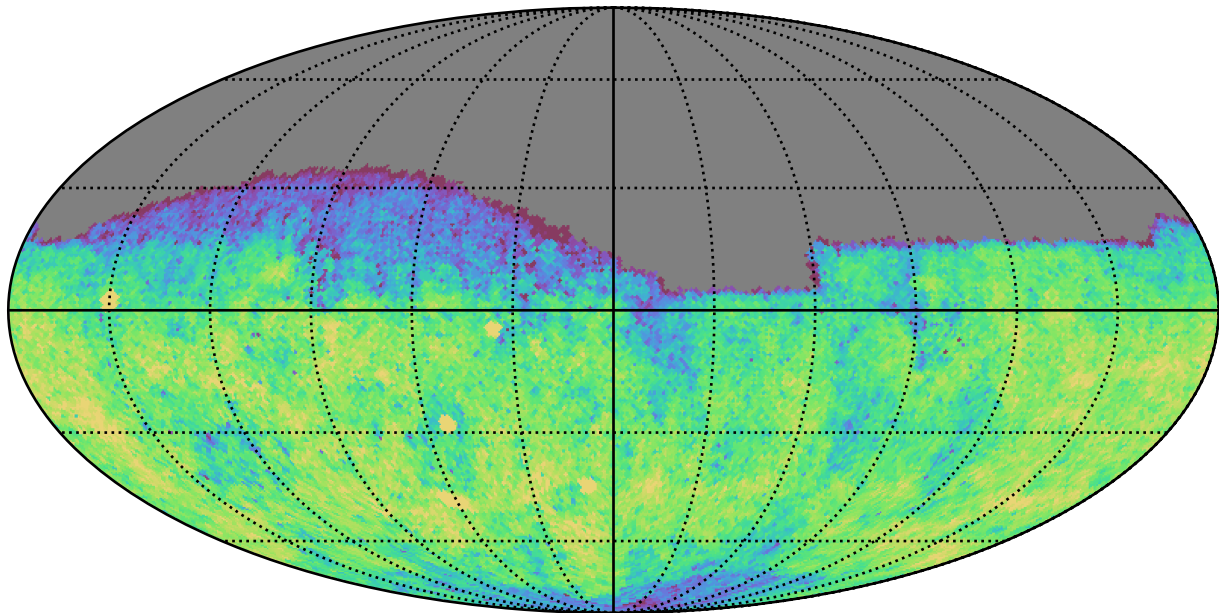
ddf_acor_sf15_lsf30_lsr50_v3.4_10yrs Yr 1 g band: CoaddM5
