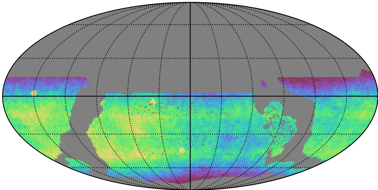
ddf_acor_sf15_lsf30_lsr50_v3.4_10yrs WFD i band: CoaddM5
