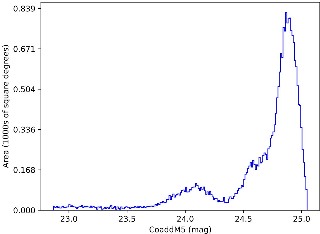
ddf_acor_sf15_lsf30_lsr50_v3.4_10yrs All sky y band: CoaddM5
