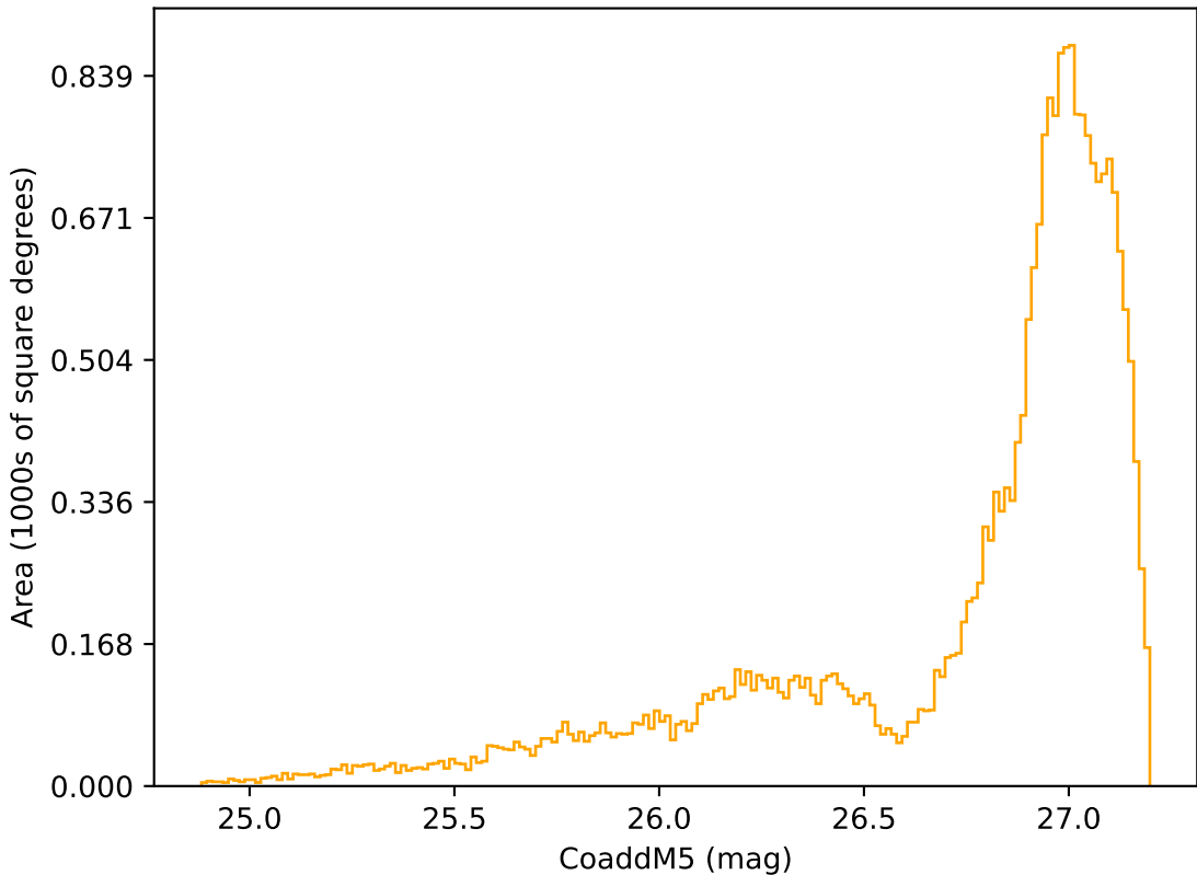
ddf_acor_sf15_lsf30_lsr50_v3.4_10yrs All sky r band: CoaddM5
