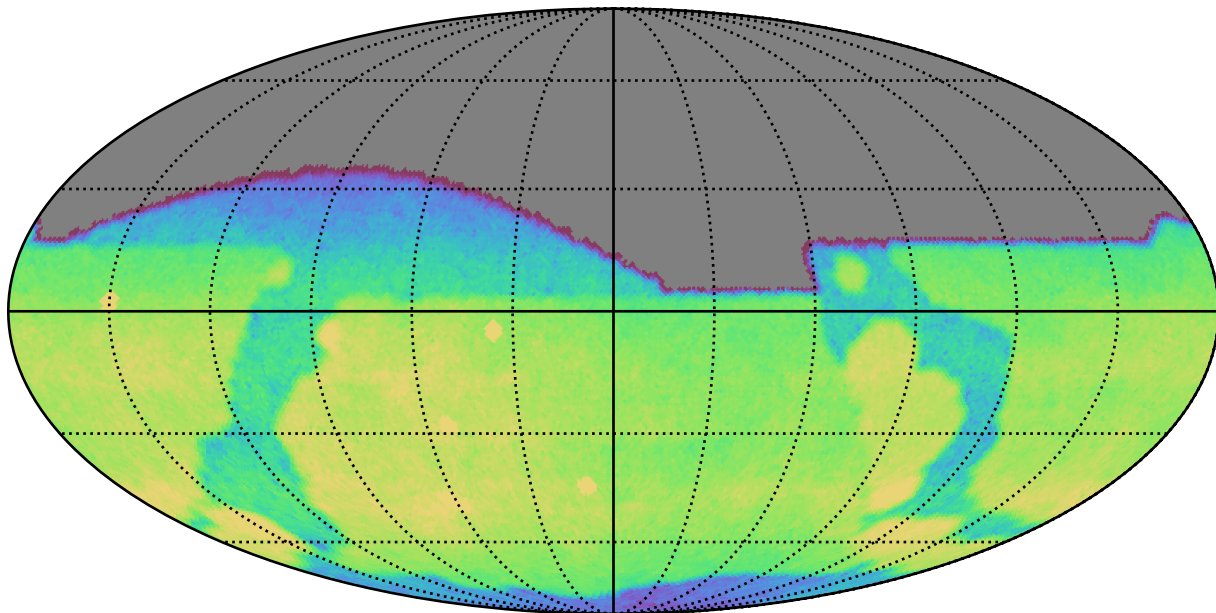
ddf_acor_sf15_lsf30_lsr50_v3.4_10yrs All sky g band: CoaddM5
