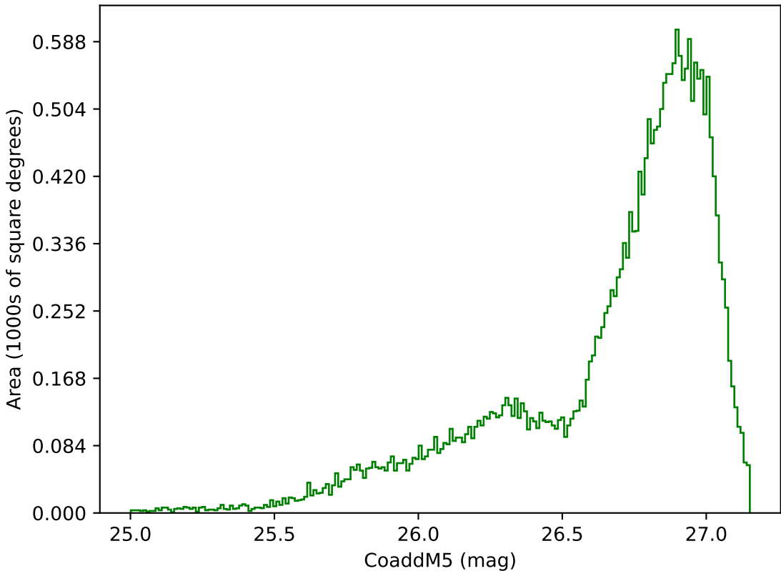
ddf_acor_sf15_lsf30_lsr50_v3.4_10yrs All sky g band: CoaddM5
