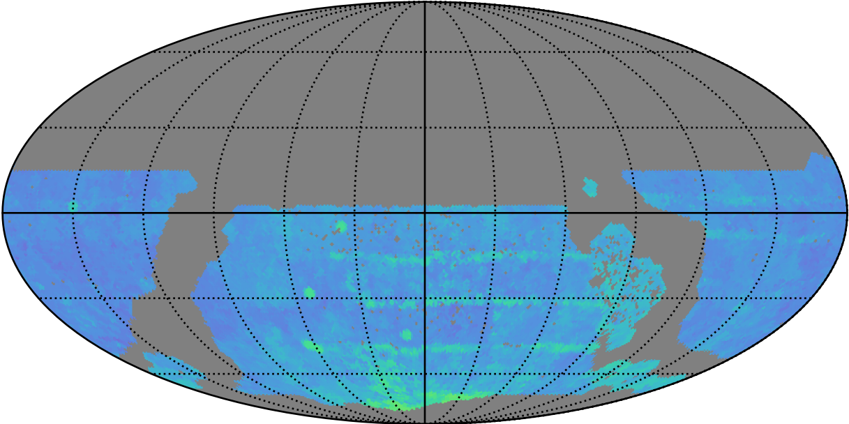
ddf_acor_sf15_lsf30_lsr50_v3.4_10yrs WFD i band: 80thPercentile Season Length
