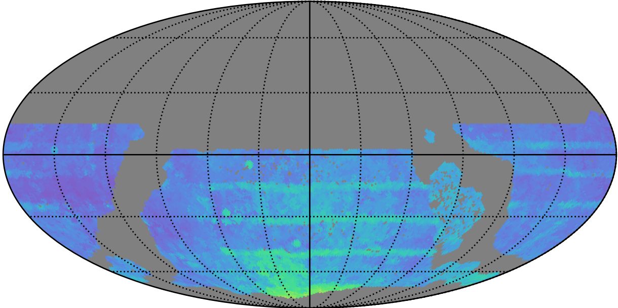
ddf_acor_sf15_lsf30_lsr50_v3.4_10yrs WFD all bands: 80thPercentile Season Length
