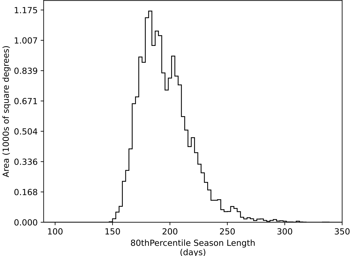
ddf_acor_sf15_lsf30_lsr50_v3.4_10yrs WFD all bands: 80thPercentile Season Length
