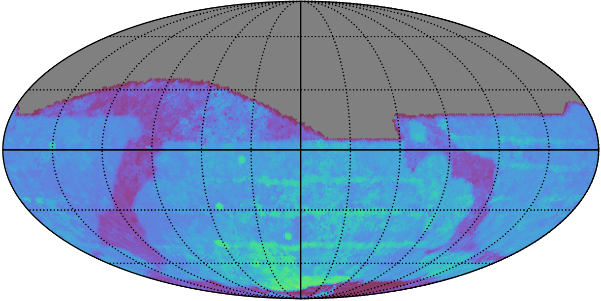
ddf_acor_sf15_lsf30_lsr50_v3.4_10yrs All sky z band: 80thPercentile Season Length
