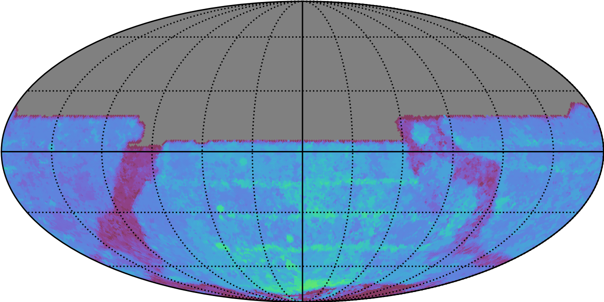
ddf_acor_sf15_lsf30_lsr50_v3.4_10yrs All sky y band: 80thPercentile Season Length
