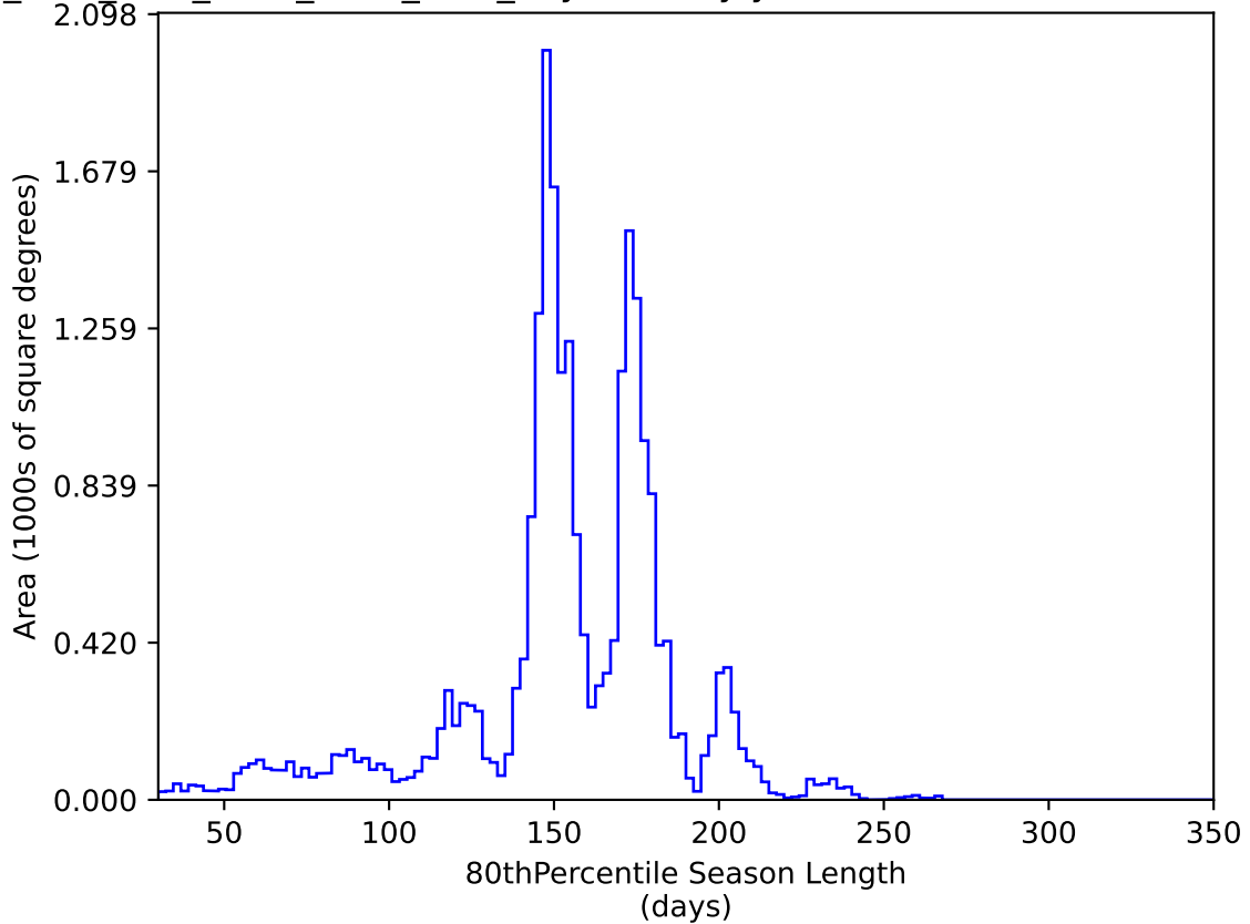
ddf_acor_sf15_lsf30_lsr50_v3.4_10yrs All sky y band: 80thPercentile Season Length
