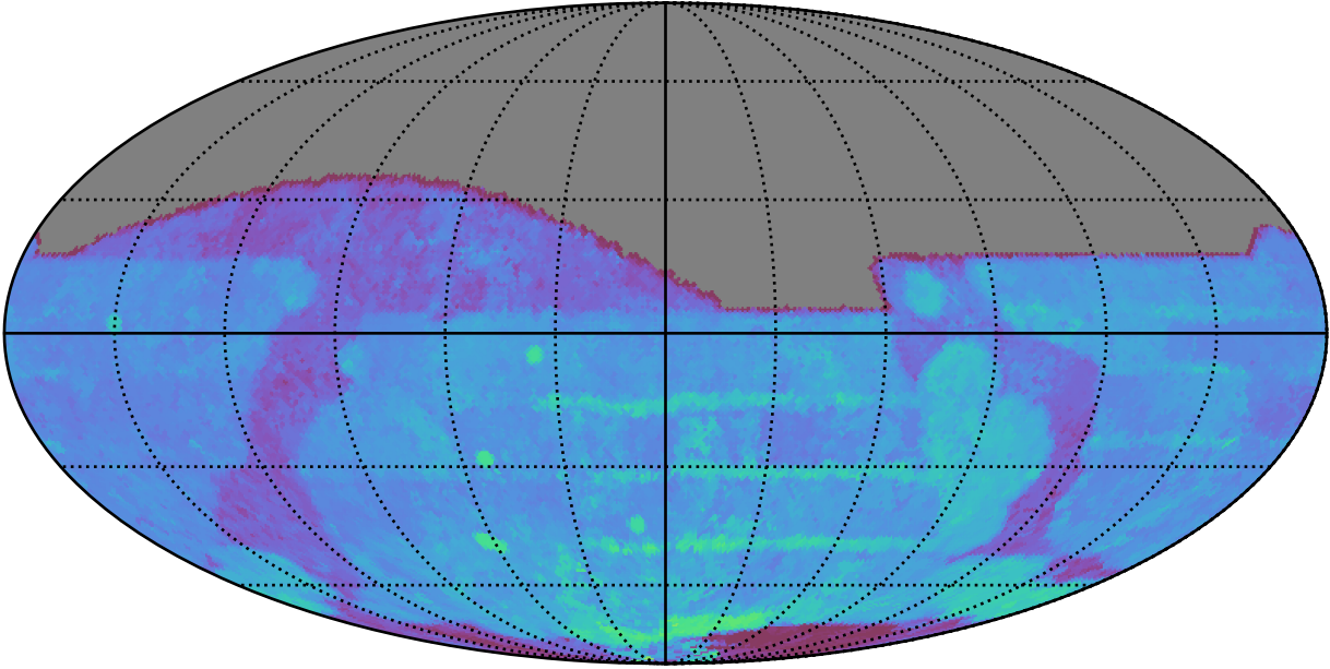
ddf_acor_sf15_lsf30_lsr50_v3.4_10yrs All sky r band: 80thPercentile Season Length
