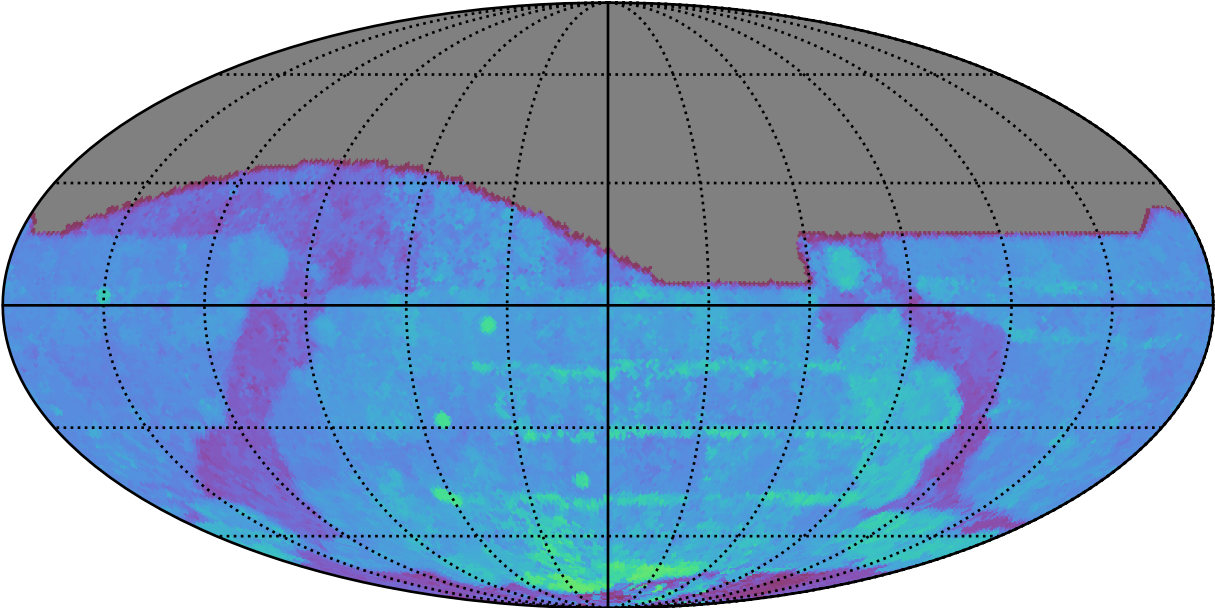
ddf_acor_sf15_lsf30_lsr50_v3.4_10yrs All sky i band: 80thPercentile Season Length
