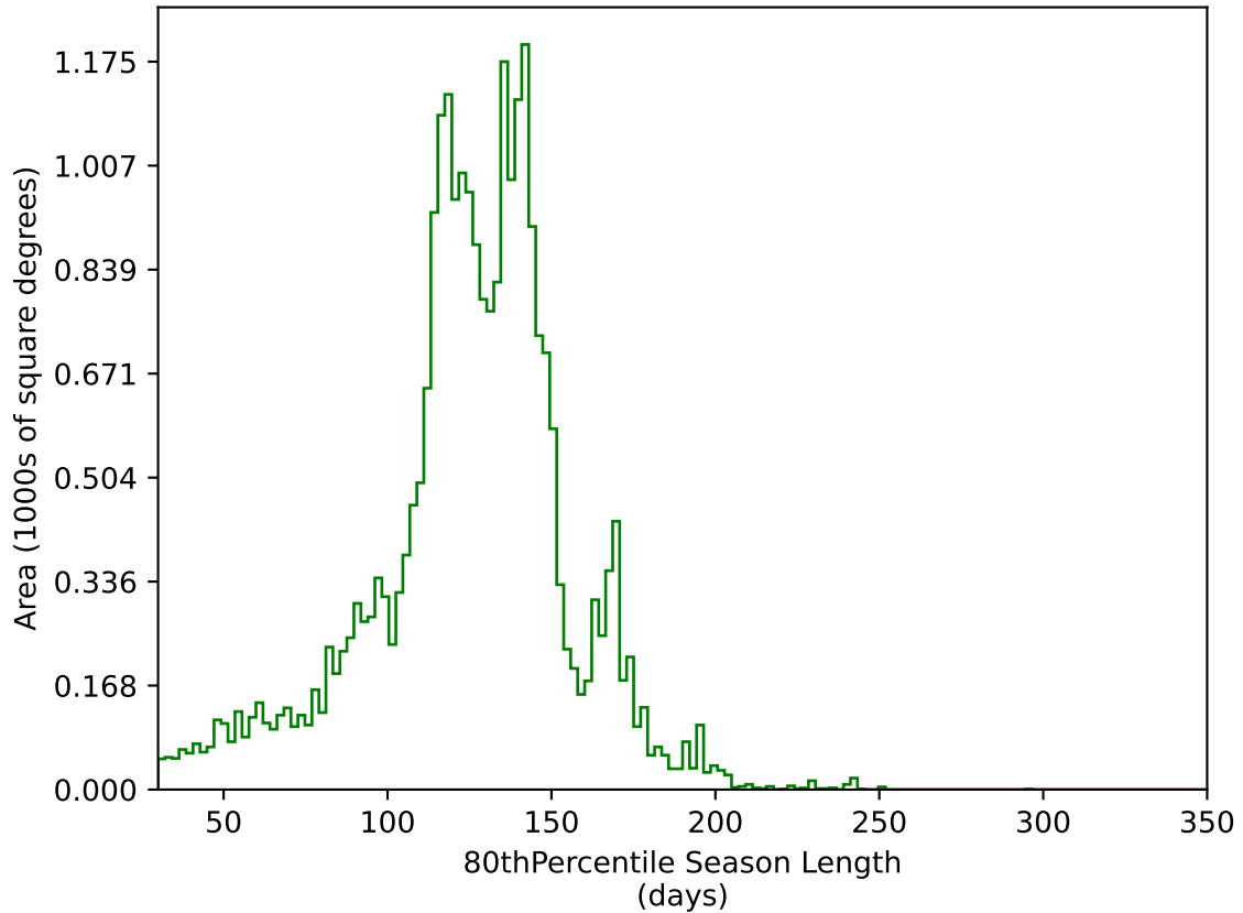
ddf_acor_sf15_lsf30_lsr50_v3.4_10yrs All sky g band: 80thPercentile Season Length
