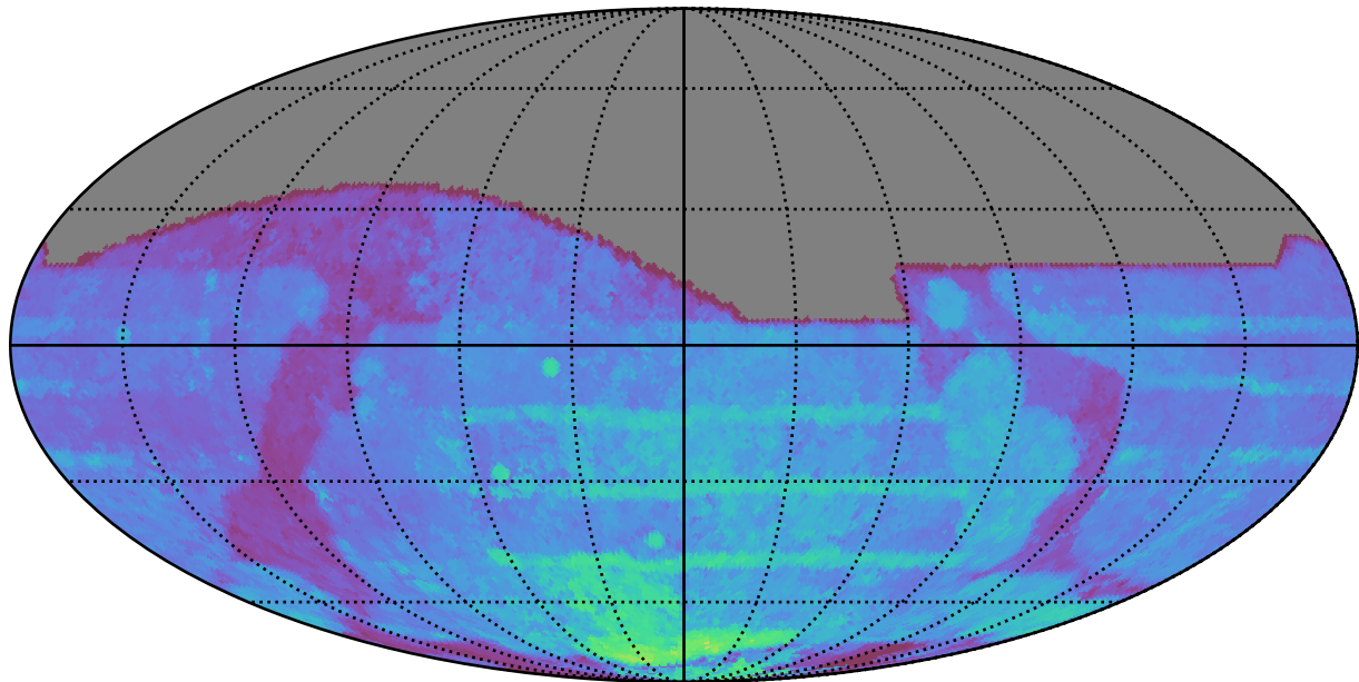
ddf_acor_sf15_lsf30_lsr50_v3.4_10yrs All sky all bands: 80thPercentile Season Length
