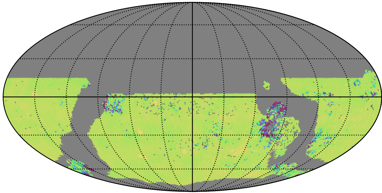
ddf_acor_sf15_lsf30_lsr50_v3.4_10yrs WFD ug bands: 75th Percentile Intranight Timespan
