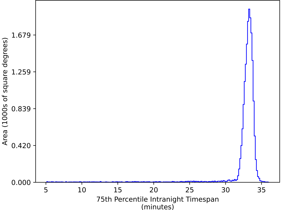
ddf_acor_sf15_lsf30_lsr50_v3.4_10yrs WFD ug bands: 75th Percentile Intranight Timespan
