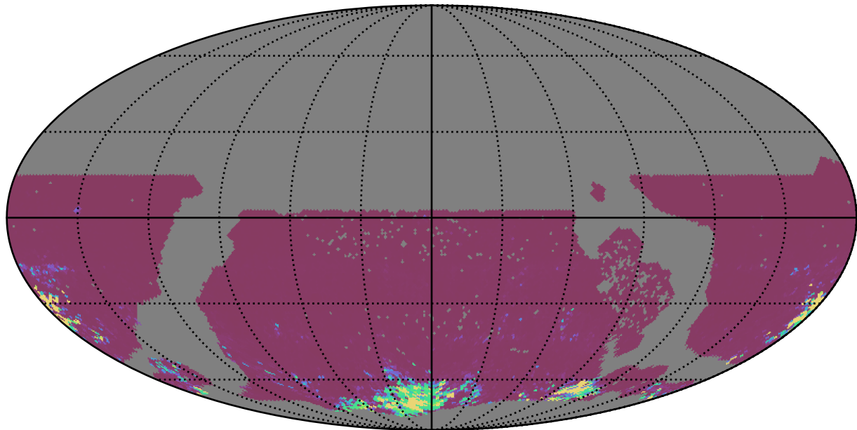
ddf_acor_sf15_lsf30_lsr50_v3.4_10yrs WFD ri bands: 75th Percentile Intranight Timespan
