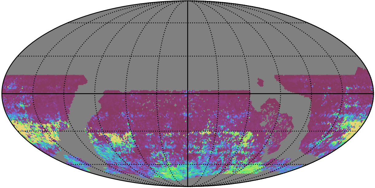
ddf_acor_sf15_ls30_lsr50_v3.4_10yrs WFD r band: 75th Percentile Intranight Timespan
