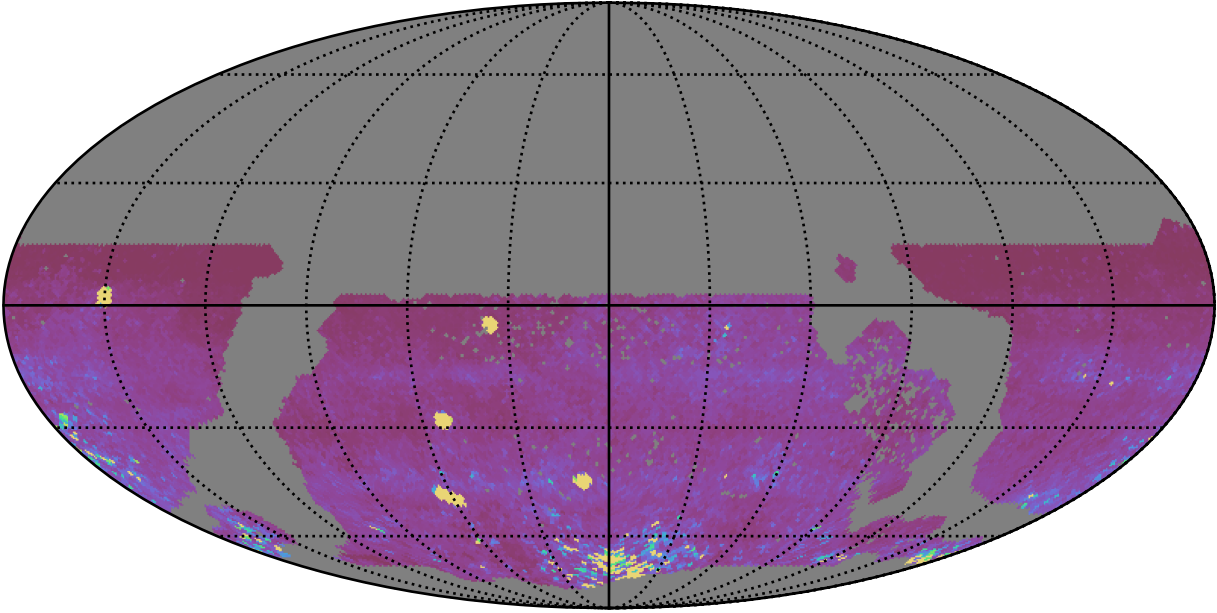
ddf_acor_sf15_lsf30_lsr50_v3.4_10yrs WFD iz bands: 75th Percentile Intranight Timespan
