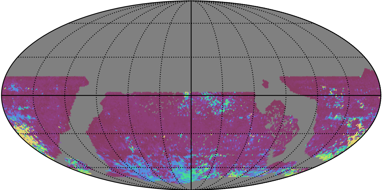
ddf_acor_sf15_lsf30_lsr50_v3.4_10yrs WFD i band: 75th Percentile Intranight Timespan
