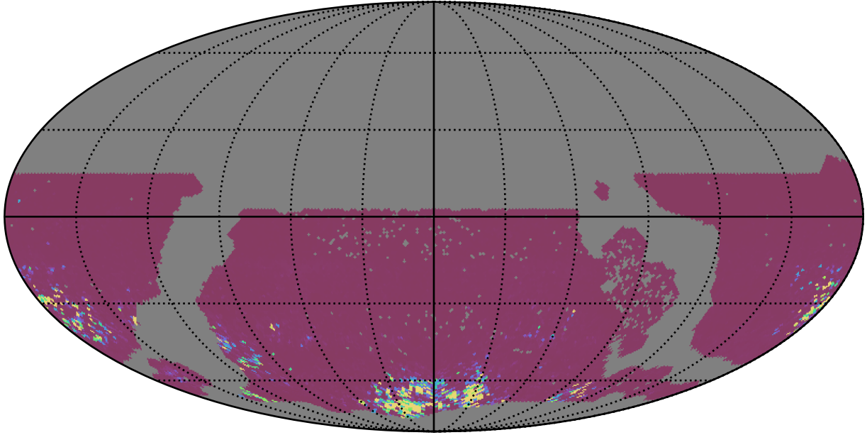
ddf_acor_sf15_lsf30_lsr50_v3.4_10yrs WFD gr bands: 75th Percentile Intranight Timespan
