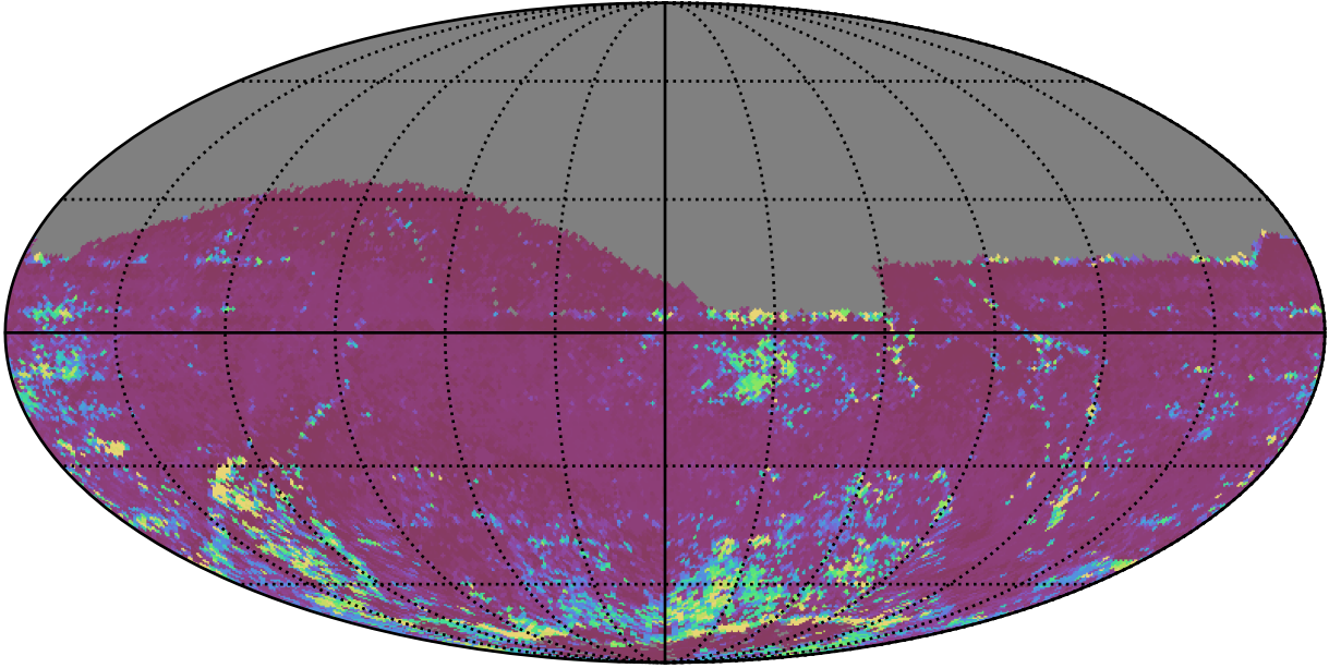
ddf_acor_sf15_lsf30_lsr50_v3.4_10yrs All sky z band: 75th Percentile Intranight Timespan
