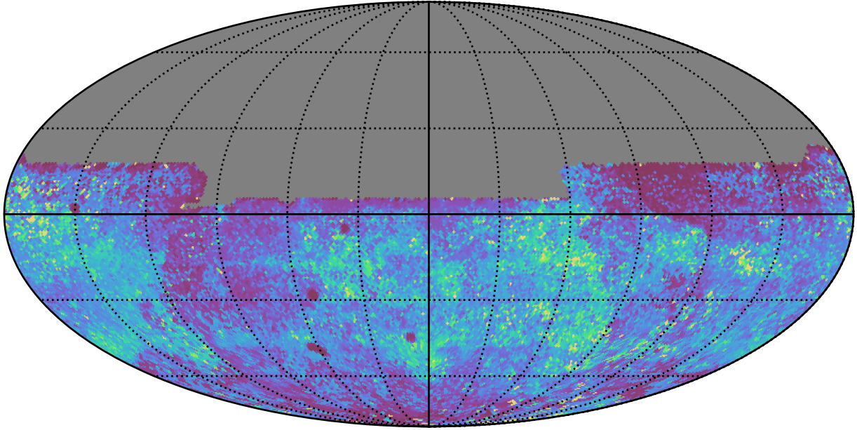
ddf_acor_sf15_lsf30_lsr50_v3.4_10yrs All sky y band: 75th Percentile Intranight Timespan
