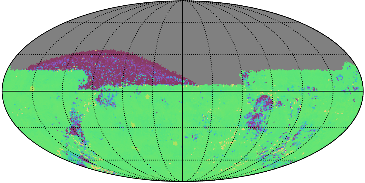
ddf_acor_sf15_lsf30_lsr50_v3.4_10yrs All sky ug bands: 75th Percentile Intranight Timespan
