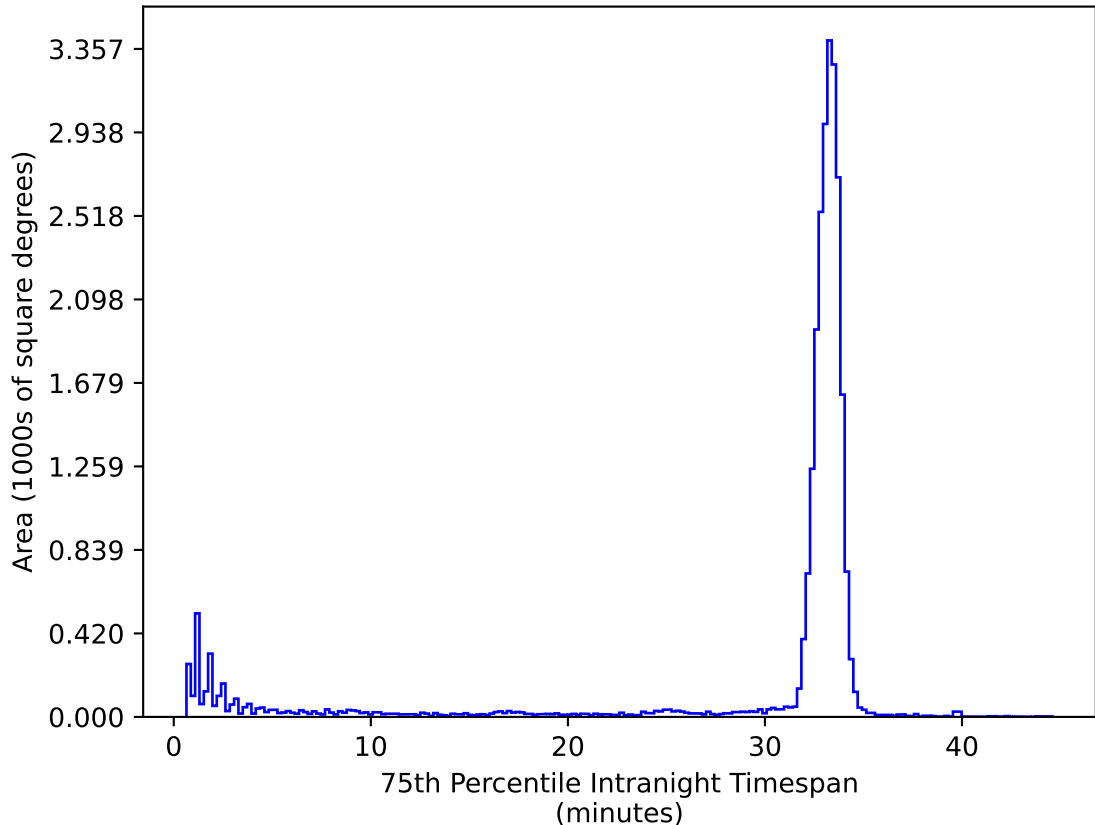
ddf_acor_sf15_lsf30_lsr50_v3.4_10yrs All sky ug bands: 75th Percentile Intranight Timespan
