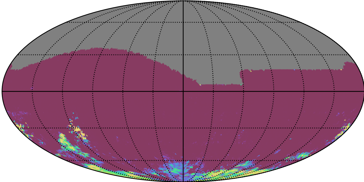
ddf_acor_sf15_lsf30_lsr50_v3.4_10yrs All sky ri bands: 75th Percentile Intranight Timespan
