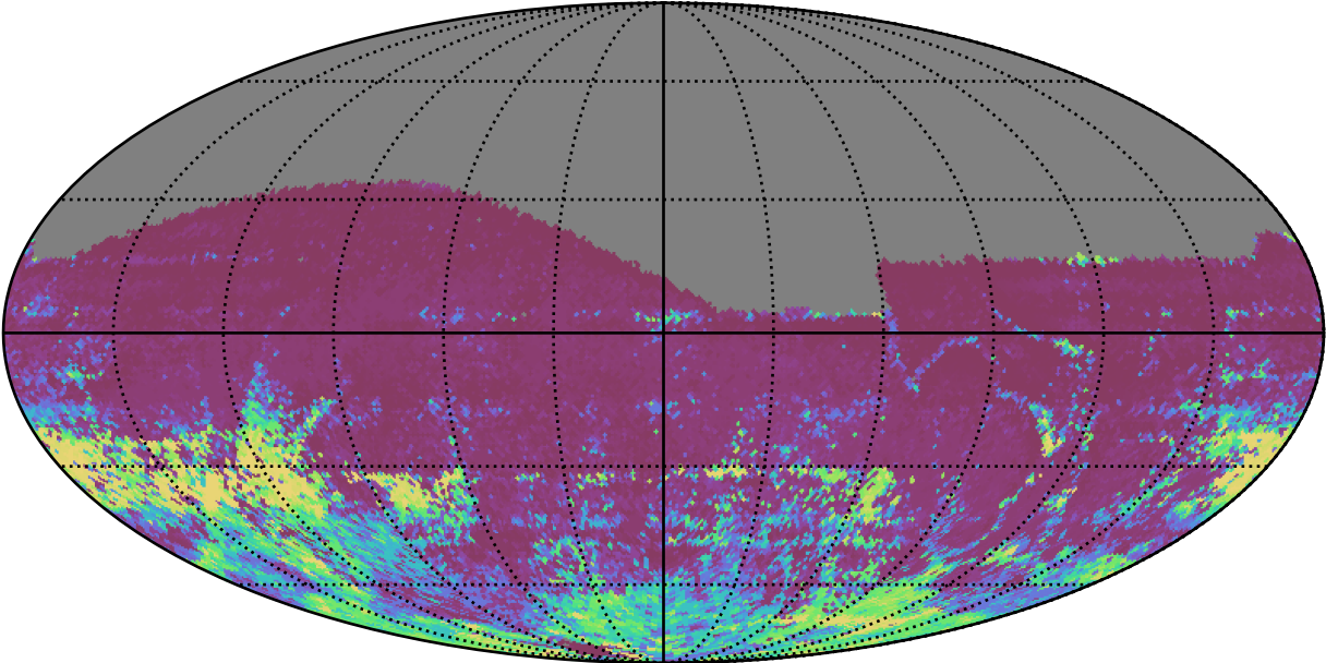
ddf_acor_sf15_lsf30_lsr50_v3.4_10yrs All sky r band: 75th Percentile Intranight Timespan
